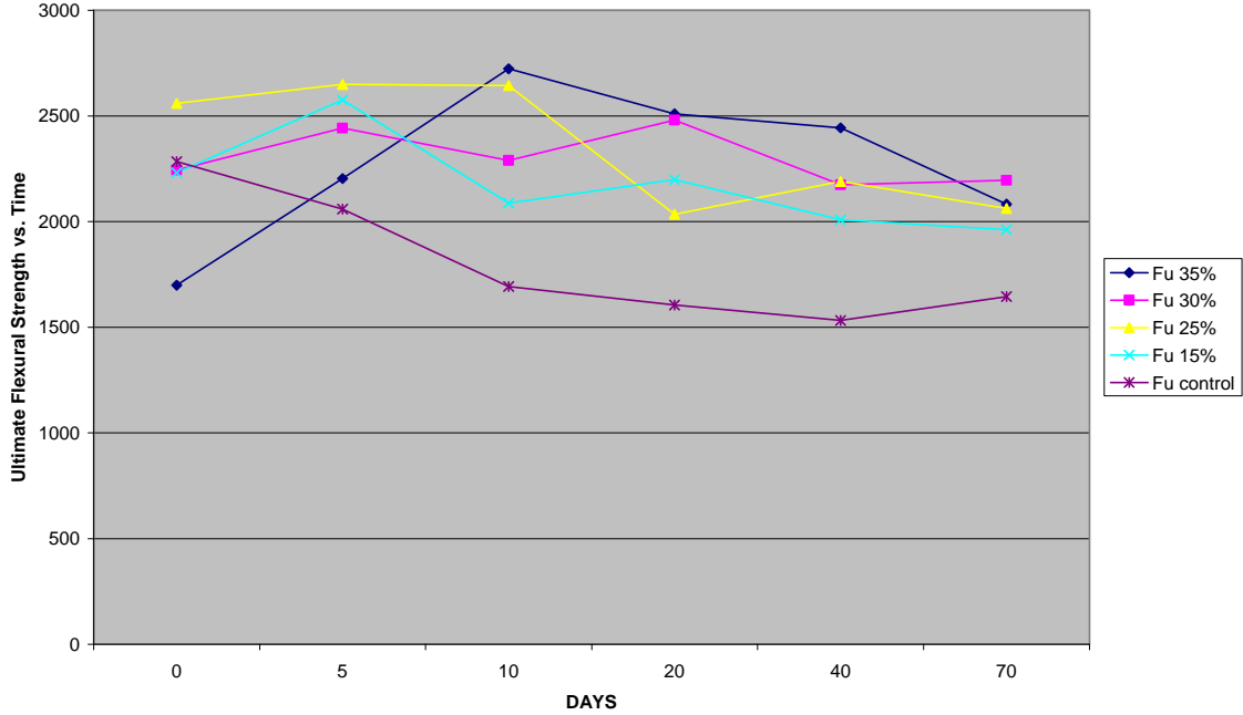
Figure 4 - Ultimate Flexural Strength vs. Time
