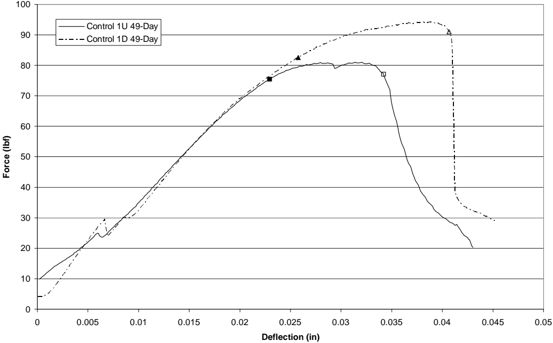
Figure 10 – Stress vs. Strain Chart at 49 Days for Control Composite
